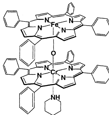
[(tpp)FeOCr(tpp)(pip)] ( II )
