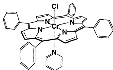
[(tpp)CrCl(py)] ( I )
